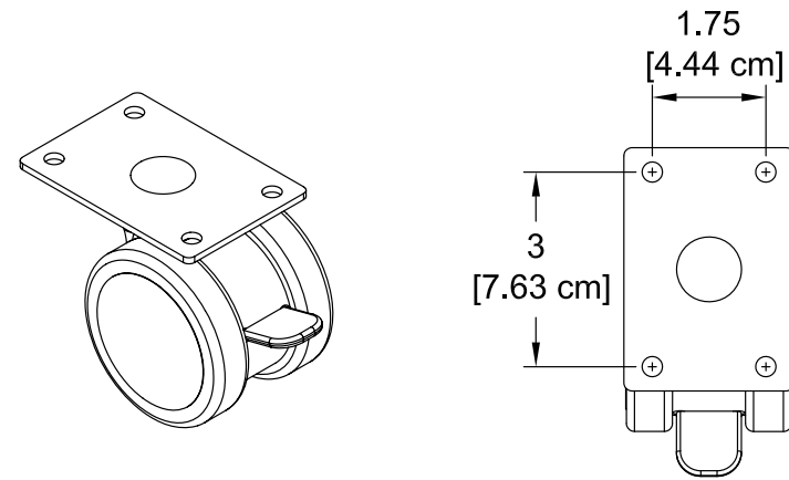
Twin-wheel casters
