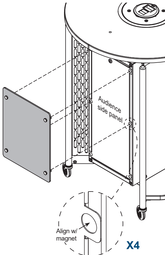
(1) 55572 Assembly
