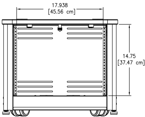
Front view (shown with front panel removed)
